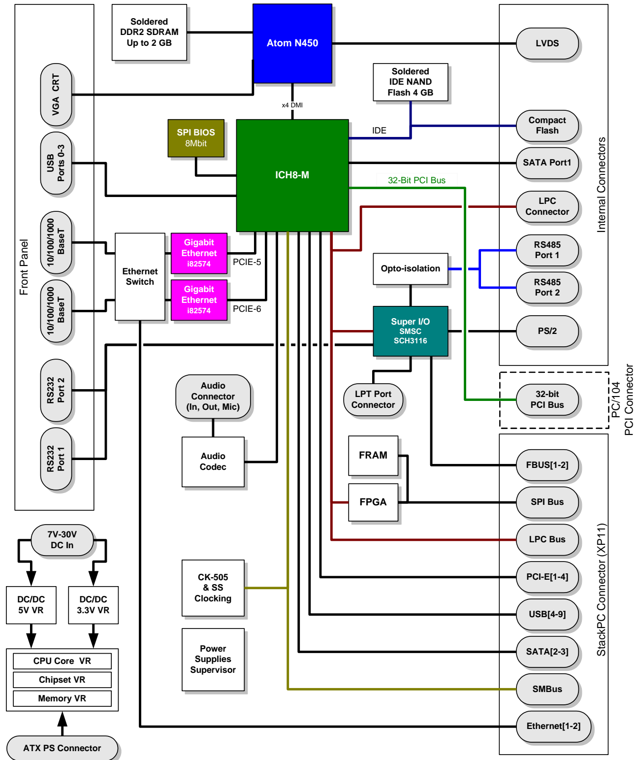
Figure 1-1: CPC805 Block Diagram
